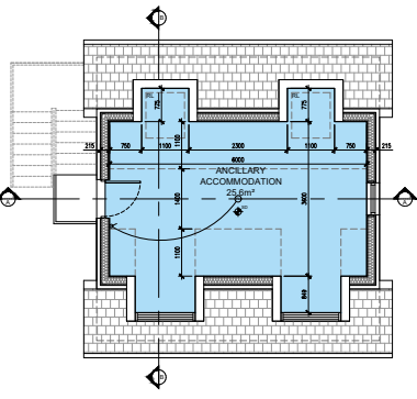
Garage First Floor Plan
